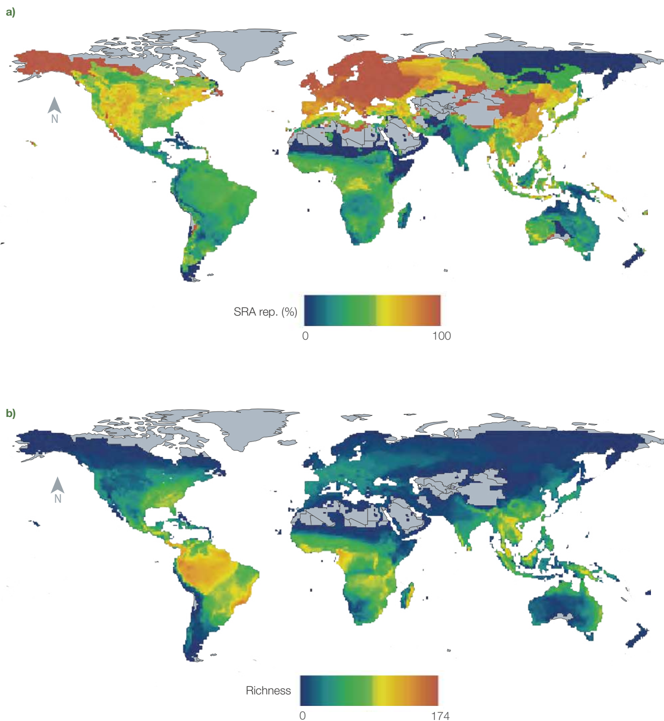
Figure 13.2: Biased geographic distribution of high-throughput sequencing effort. a) Percentage of amphibian species sequenced and b) amphibian species richness. Distribution polygons from the Red List and SRA records were spatially joined at ~10km resolution in ArcGIS® software (ESRI, Redlands, CA) to estimate the species richness and the percentage of occurring species with high-throughput sequence information. Source: Data from SRA ( www.ncbi.nlm.nih.gov/sra , accessed in January 2021) and the Red List ( www.iucnredlist.org/ , accessed in January 2021).
