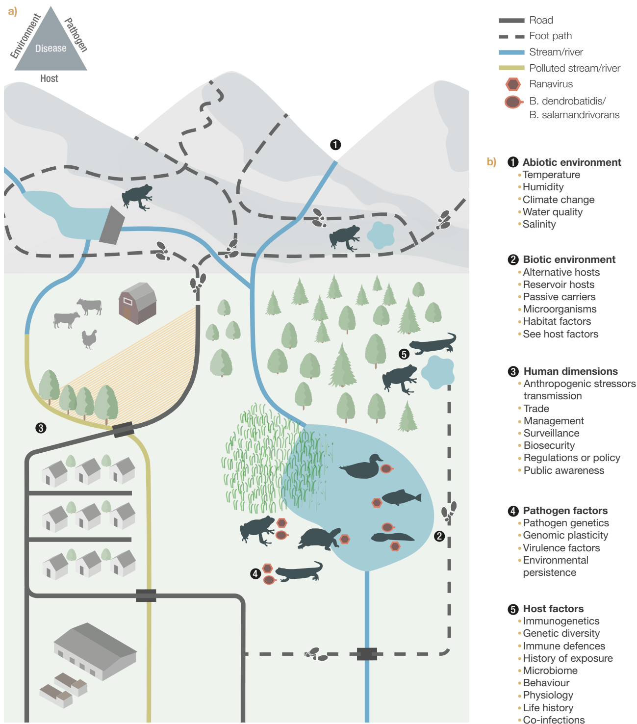
Figure 6.1: Schematic representation of specific elements of the disease triangle a) . Disease may develop where conducive factors of the environment (abiotic, biotic, human dimensions), pathogen, and host overlap b) . Source: Inspired by Fisher & Garner (2020).
