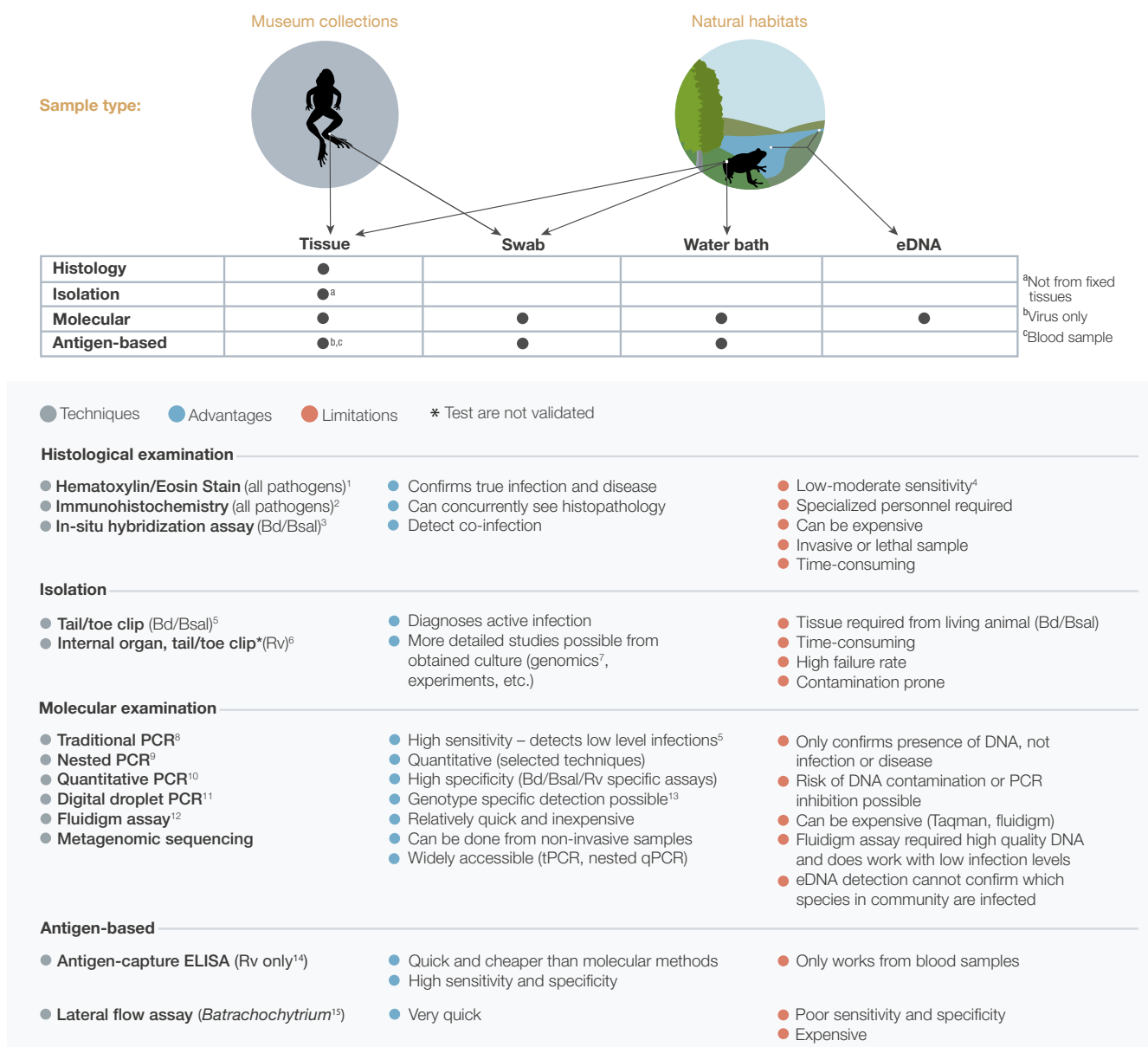
Figure 6.2: Diagnostic tools for amphibian pathogens and disease. Diagnostic screening techniques can be applied to museum specimens, field-caught individuals as well as environmental substrates (e.g. water). Histological, isolation, molecular and antigen-based tools are available, each with their own set of advantages and disadvantages. Histological examination is still the only method capable of diagnosing clinical infection and disease, but has from low to moderate sensitivity and is costly. Isolation of pathogens can be difficult, but is essential for developing a deeper understanding of pathogens, their ecology, physiology and behaviour. Molecular tools offer non-invasive sampling methods and high sensitivity for detecting genetic material of pathogens, but quantitative PCR (qPCR) based methods don't come without important caveats. There can be wide variation in quantification according to laboratory methods making direct comparisons across studies difficult. This variation may be attributed to using different standard cultures/strains of Bd, different qPCR cycling parameters and molecular techniques, and different DNA extraction techniques (Bletz, Rebollar & Harris, 2015; Brannelly et al., 2020). There has been an attempt to standardise across studies using Bd intergenic transcribed spacer (ITS) copy number standards (Longo et al., 2013; Rebollar et al., 2017); however, with variation in ITS within the fungal genomes the biological meaning can be skewed (e.g. 1000 ITS copies could be equivalent to 2 zoospores if copy number is 500, or 200 zoospores if the copy number is 5). It is additionally important to understand the detection limits of molecular techniques like qPCR. Low and inconsistent qPCR positives may be false positives, and mutations in the ITS region at the Taqman probe binding site in certain regions, such as Asia, can lead to false negatives (Mutnale et al., 2018). This caveat is also true for qPCR methods used to detect ranaviral DNA (Wynne et al., 2020). Development of the lateral-flow assay by Dillon et al. (2017) shows some promise; however, this assay lacks specificity (it cross-detects related fungi) and sensitivity (it fails to detect low loads). Source: 1 Berger et al. 1999, Forzan et al. 2017; 2 Olsen et al. 2004, Jerret et al. 2015; 3 Ossiboff et al. 2019, Forzan et al. 2019; 4 Kruger et al. 2006; 5 Cook et al. 2018; 6 Granoff et al. 1965, Balseiro et al. 2009; 7 Rosenblum et al. 2008, O'Hanlon et al. 2018; 8 Annis et al. 2004; 9 Goka et al. 2009; 10 Boyle et al. 2004, Bloi et al. 2013, Standish et al. 2018; 11 Pinheiro et al. 2012; 12 Byrne et al. 2019; 13 Ghosh et al. 2020; 14 Kim et al. 2015; 15 Dillon et al. 2017.
